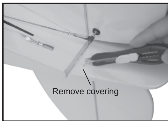
Control horn of elevator.
