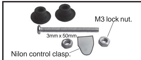
Control horn of elevator.
