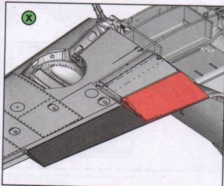
Radiator flap closed, wing flaps retracted
