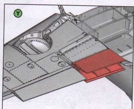
Radiator flap open, wing flaps retracted
