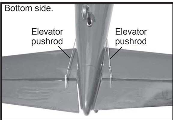
Plastic parts of elevator pushrod.
